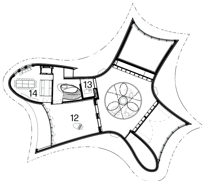
Obergeschoss (OG)
