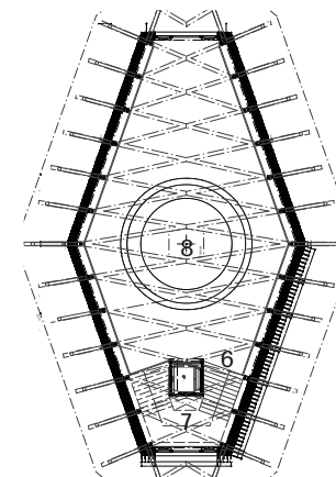
Obergeschoss (OG)
